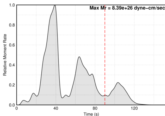
Figura 2 Relative Moment Ratio (Fuente: extraído de (United States Geological Survey (USGS), 2018)).
